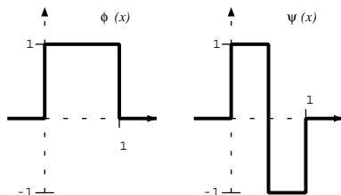
FIGURE 13. The Haar scaling function and wavelet.
