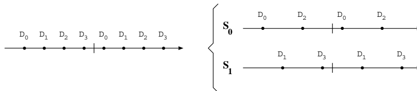
FIGURE 21. TCQ sets and supersets
