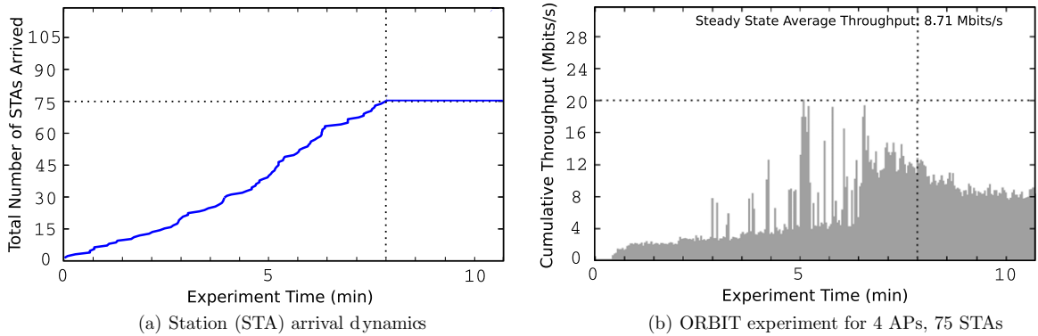
Fig. 4. System performance for the most general case: multi-cell with many clients using realistic traffic and arrival patterns.
