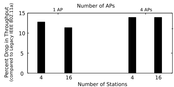
Fig. 12. Default value for AIFSN parameter of IEEE 802.11e Best Effort queue results in decreasing throughput for bulk data traffic, even in the absence of any multimedia traffic.
