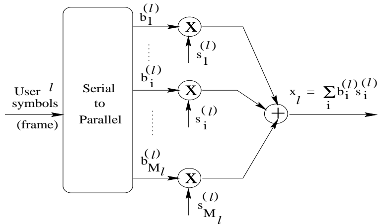
Figure 1: Multicode CDMA approach for sending frames of information. Each symbol in the frame is assigned a codeword (signature sequence) and the resulting signal \mathbf{x} is a superposition of codewords scaled by their corresponding information symbols. Our problem will be to find optimal \{s_{ij}\} .
