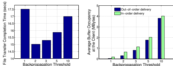
Fig. 7: Effect of variation of H on throughput and reordering at the application
