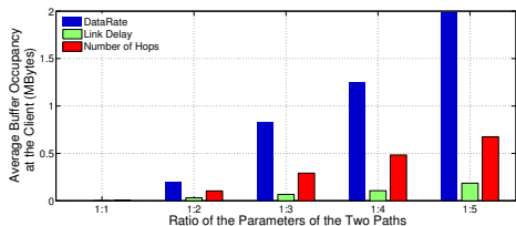
Fig. 5: Effect of link bandwidth, delay and number of hops on the reorder buffer requirements at the client
