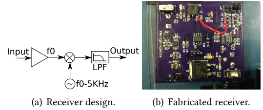
Figure 10: Touch receiver.
