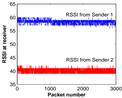
(b) RSSI at receiver for each sender
