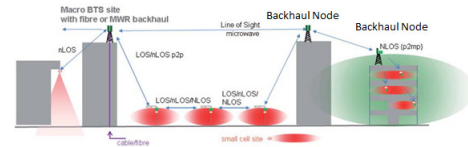
Fig. 1. The macrocell is located at the second building from the left and it has fiber connection. The red bubbles denote coverage of the small cells. The small cells located at the left side can directly communicate with the macrocell. The small cells located at the right side do not have good one-hop wireless links with the macrocell and require routing through backhaul nodes to reach the macrocell. This figure is reproduced from [7]
