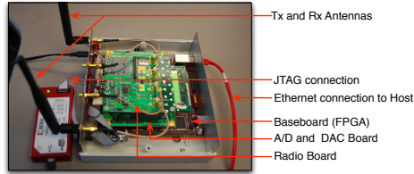
Fig. 5. SDR prototype using Virtex-V FPGA
